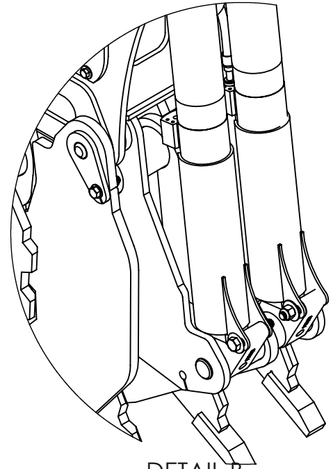
DETAIL B CYLINDER GAURDS SCALE 1 : 12
