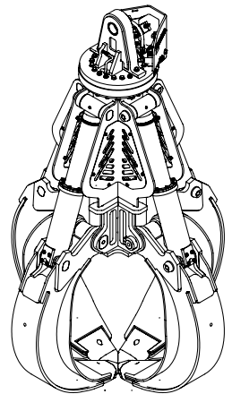
REPLACEABLE TIPS / FORGED TIPS
